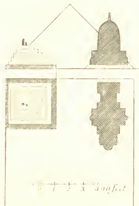
[99] Comparative size of Birs Nimroud, the Great Pyramid of Ghiza, and St. Paul's Cathedral.
